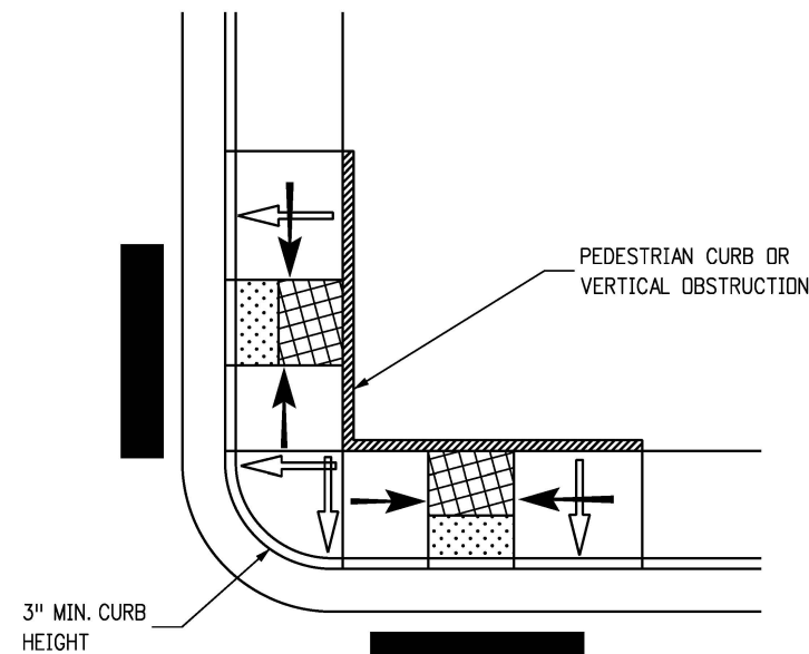
TYPE 2 RAMP SMALL RADIUS (3" REDUCED CURB)
