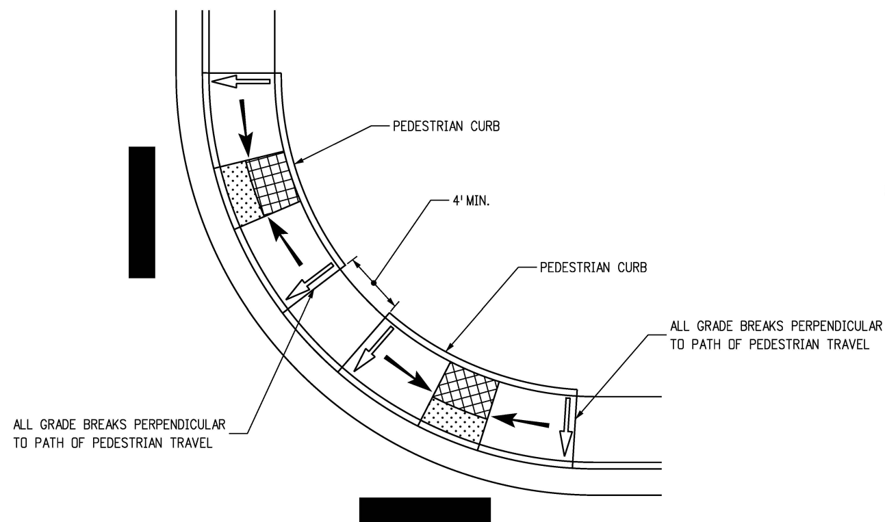
TYPE 2 RAMP LARGE RADIUS
